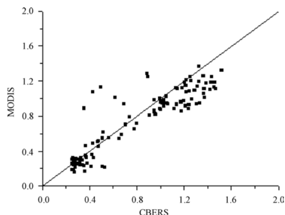
Fig. 4 Comparison on the aerosol optical depth (AOD) between CBERS02B and MODIS
